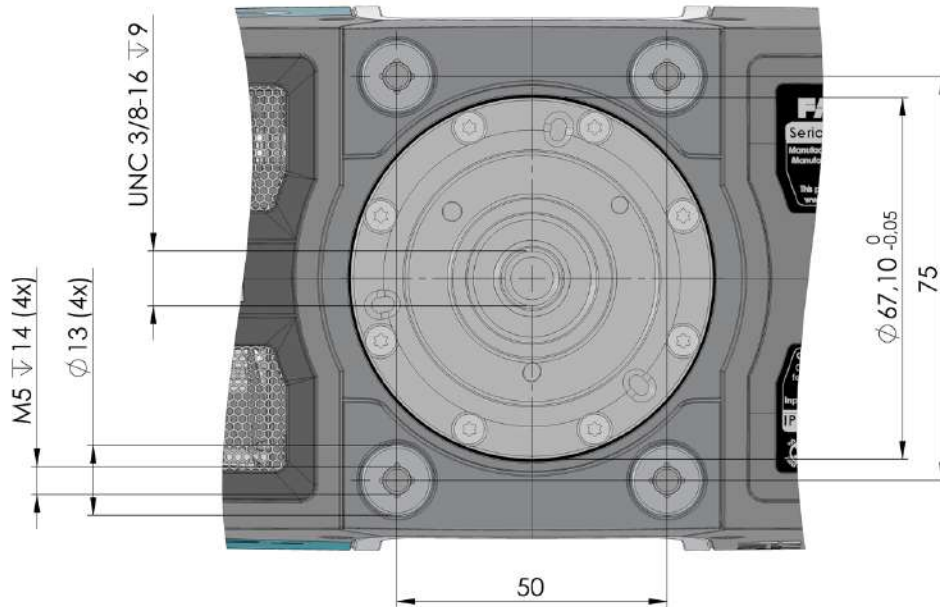
Figure 9-2 Scanner mount
