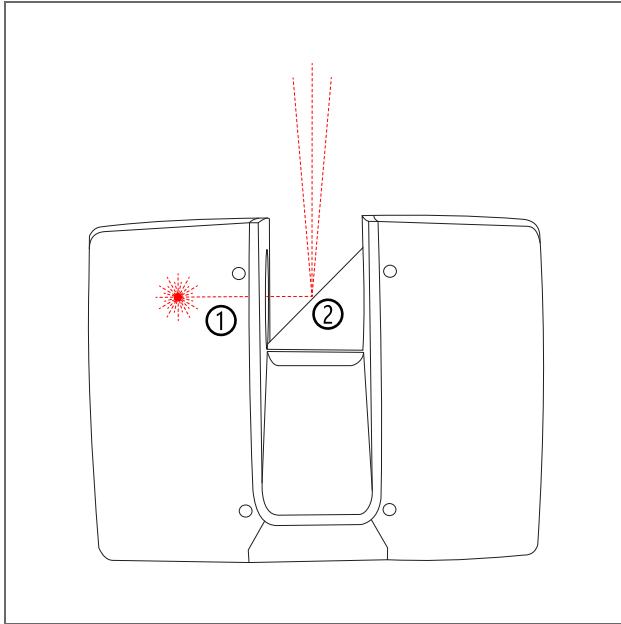
Figure 2-2 Laser Deflection
